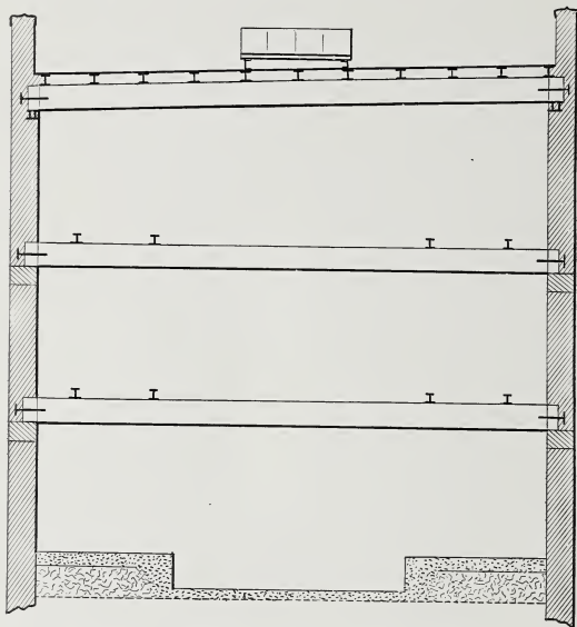
FIG. 48.—Section of a Varnish Storage-Building.
